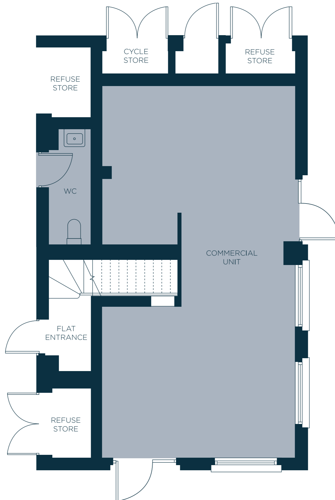
UNIT FLOOR PLAN
